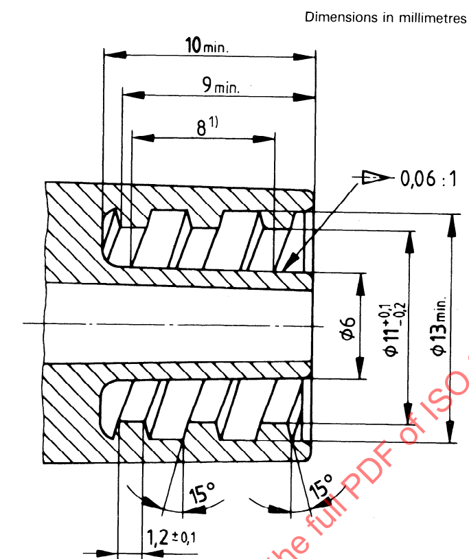
Figure 1 — Main fitting dimensions of blood inlet and outlet connections
