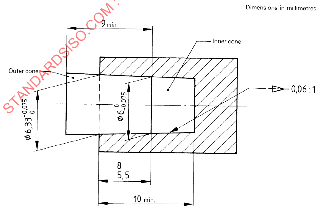
Figure 2 — Length of engagement of male and female cones of blood inlet and outlet connectors
