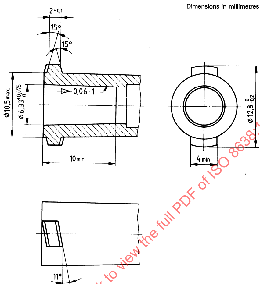
Figure 1 — Main fitting dimensions of extracorporeal circuit connector to blood ports of haemodialyser, haemofilter or haemoconcentrator
