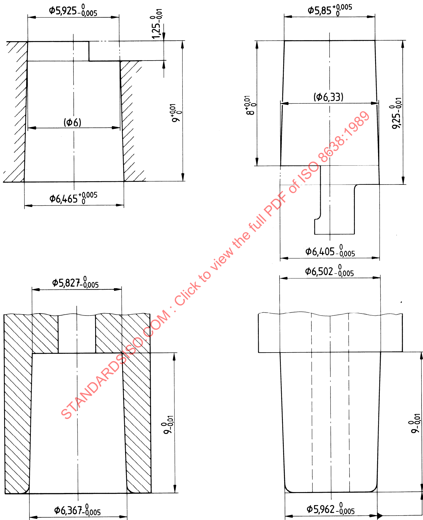
Figure 3 — Details of 6 % taper test fitting for connector to haemodialyser, haemofilter or haemoconcentrator blood port
