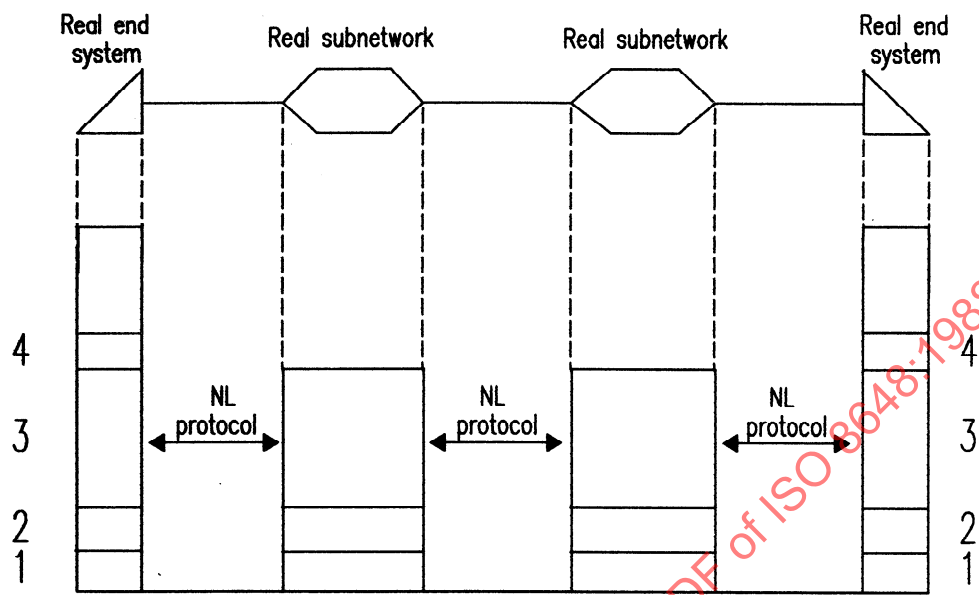
a) Direct connection without separate interworking units
