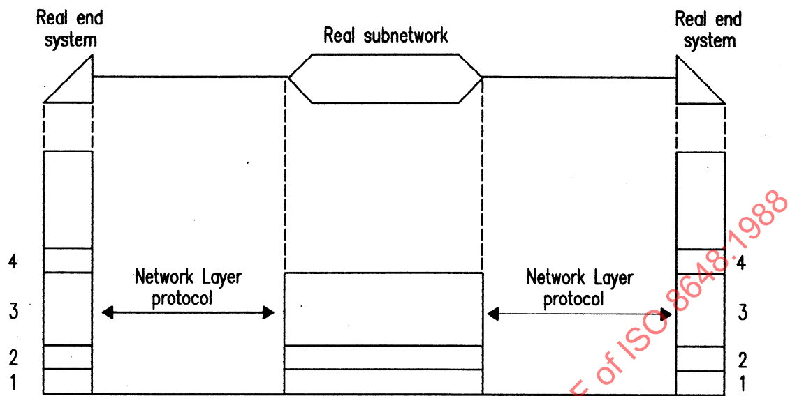
a) Use of a single Network Layer protocol
