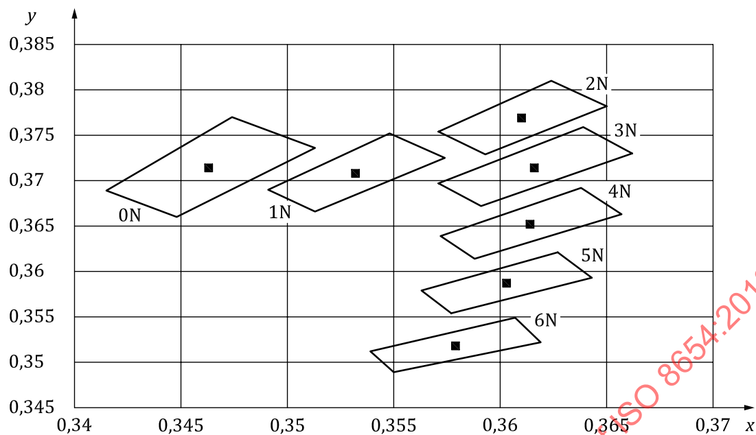
Figure 1 — xy tolerances according to Table 2
