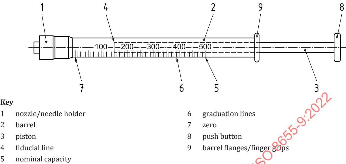
Figure 1 — Manually operated precision laboratory syringe
