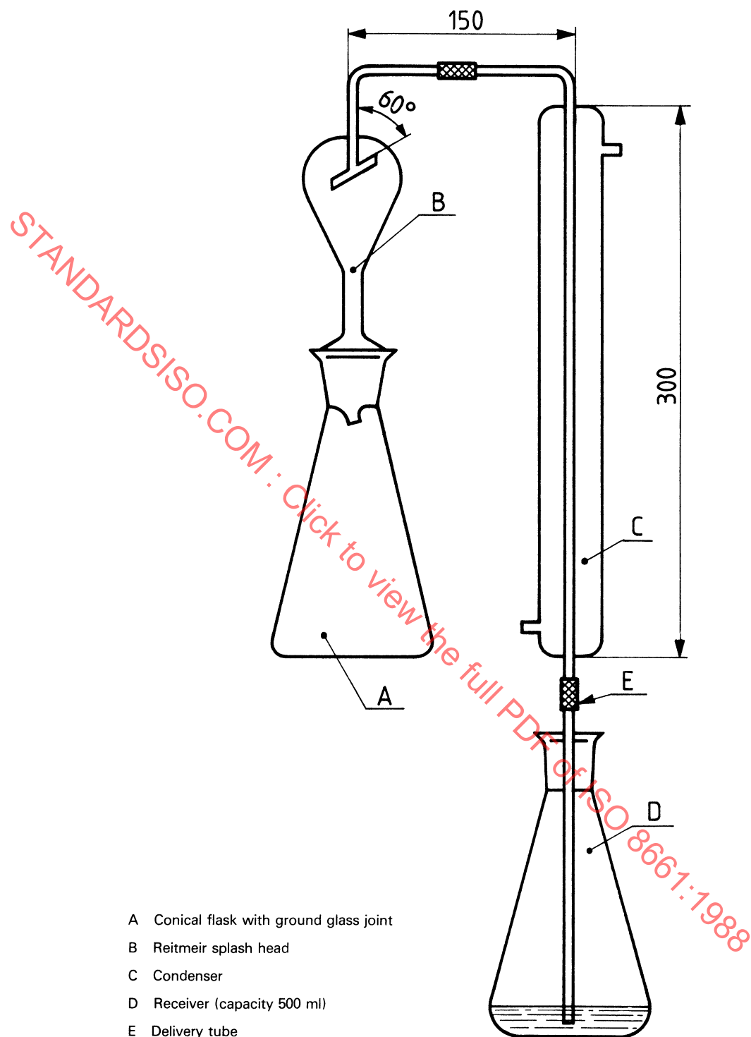
Figure 1 — Distillation apparatus
