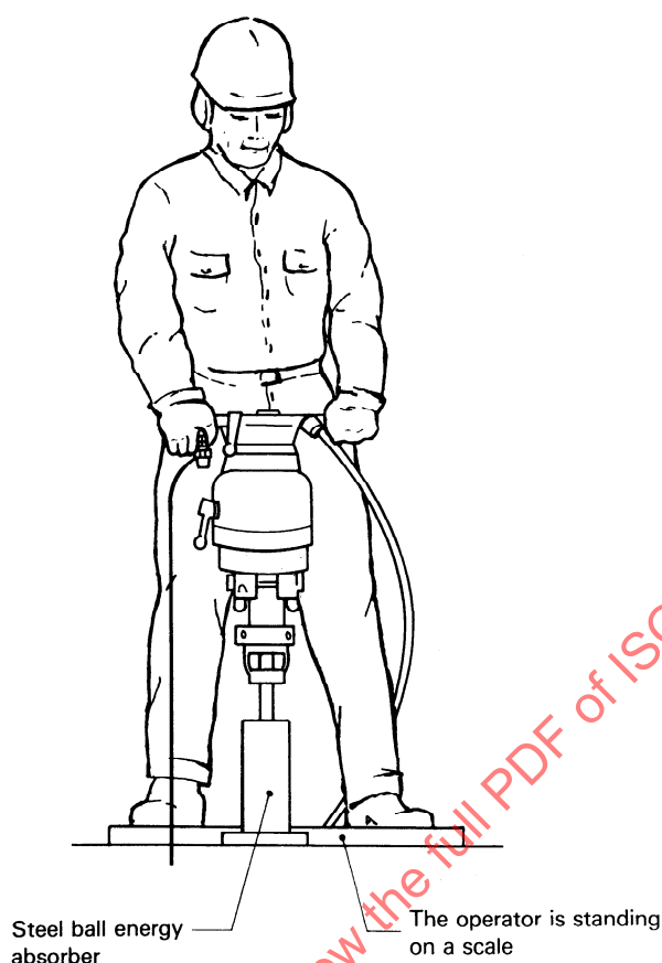
Figure 3 — Working position of operator — Rock drill
