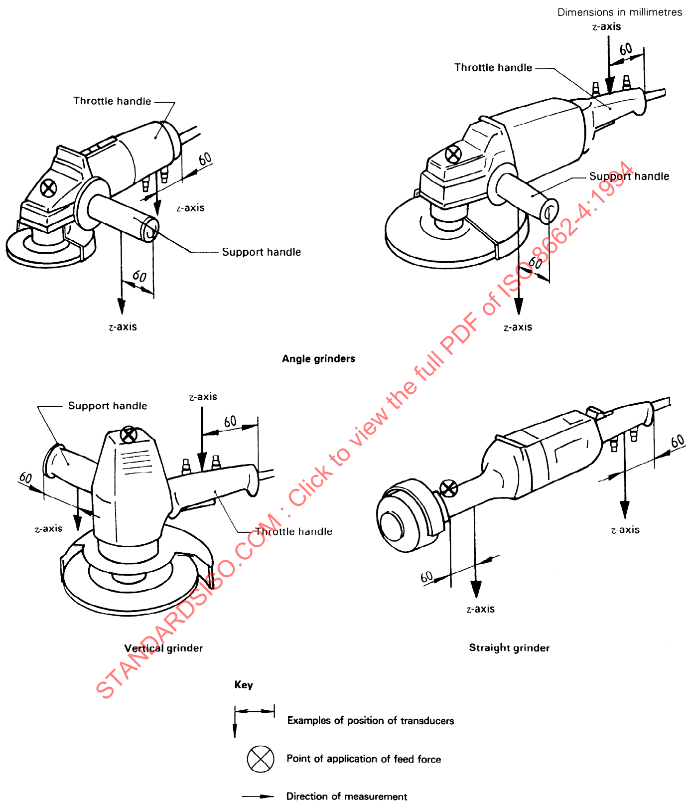
Figure 1 — Measurement directions, examples of position of transducers and application of feed force
