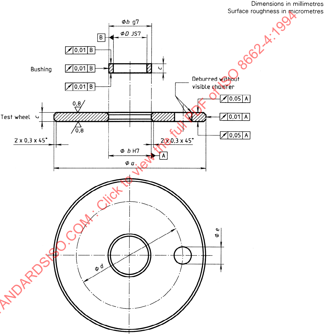
Figure 4 — Specifications of test wheel and bushing
