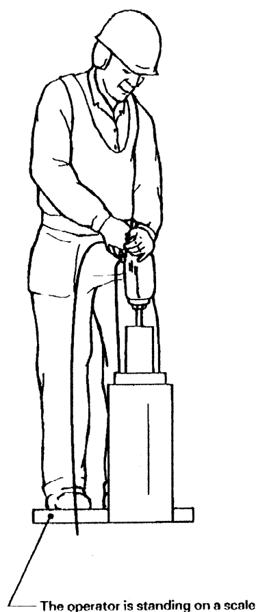
Figure 3 — Working position of operator — Pick hammer
