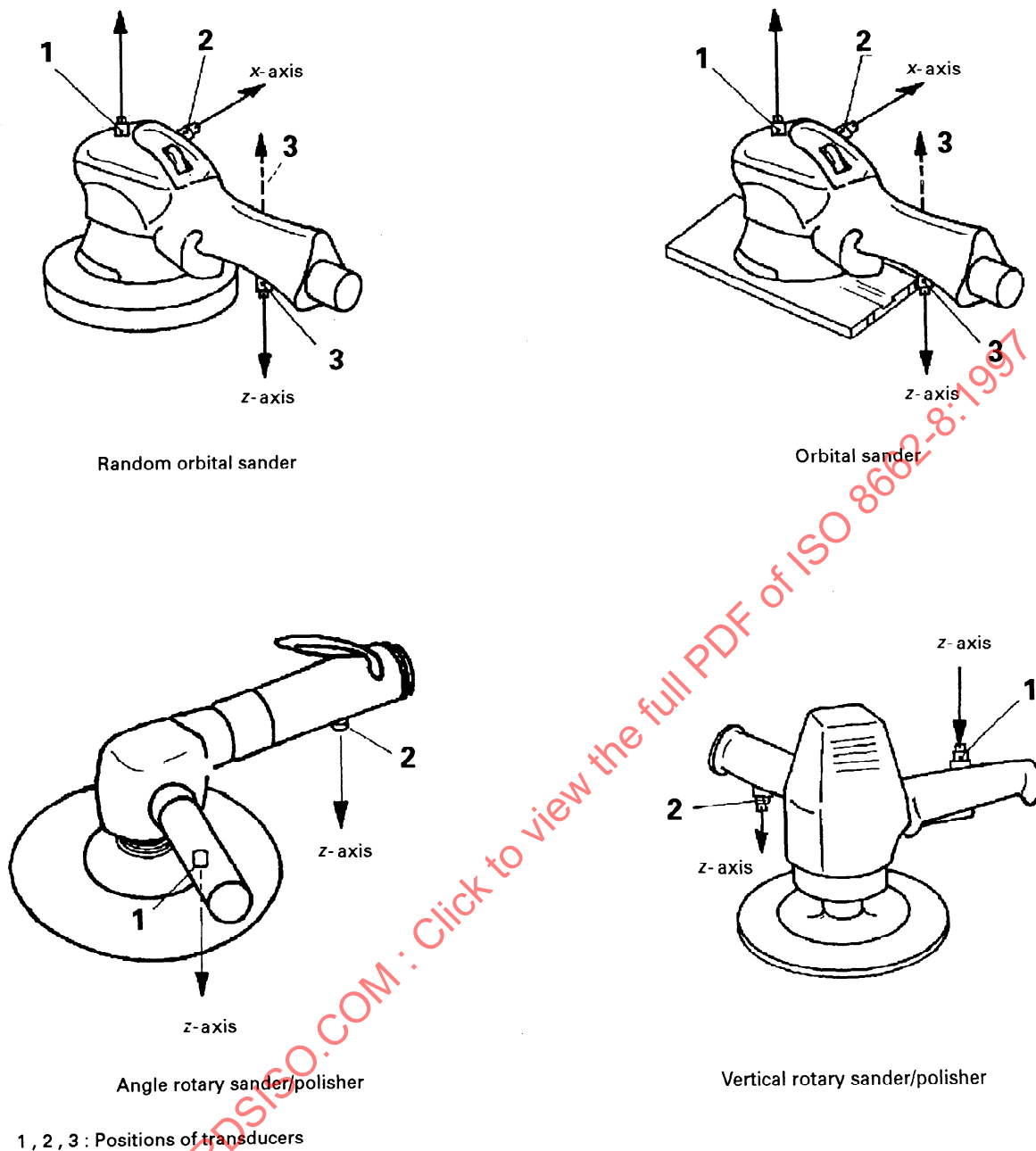
Figure 2 — Measurement directions and examples of positions of transducers
