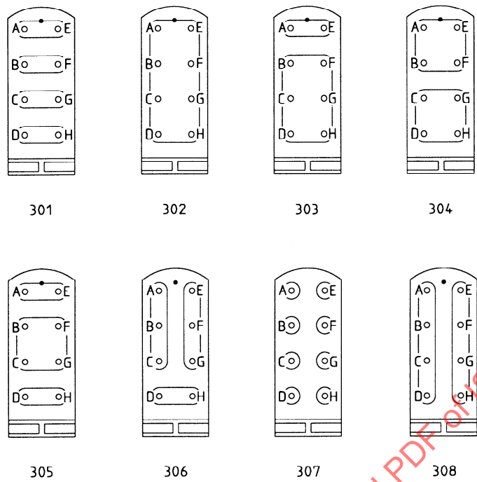
Figure 17 — Size C modules
