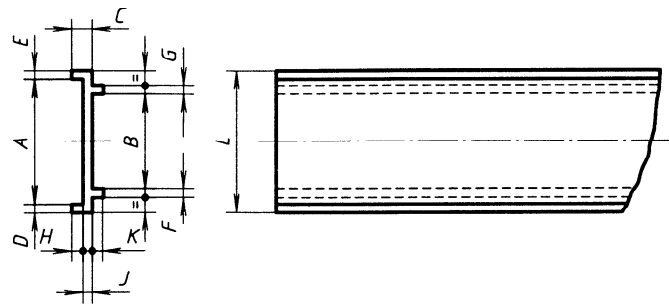
Figure 6 — Frame for feedthrough module: P4
