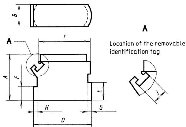
Figure 1 — Feedback module
