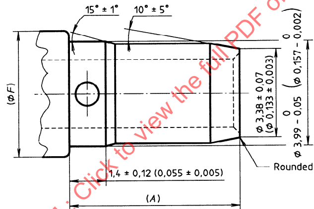
Figure 12 — Detail of the crimping shank of the size 12 contact
