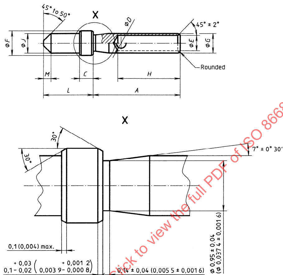
Figure 9 — Contact, size 22
