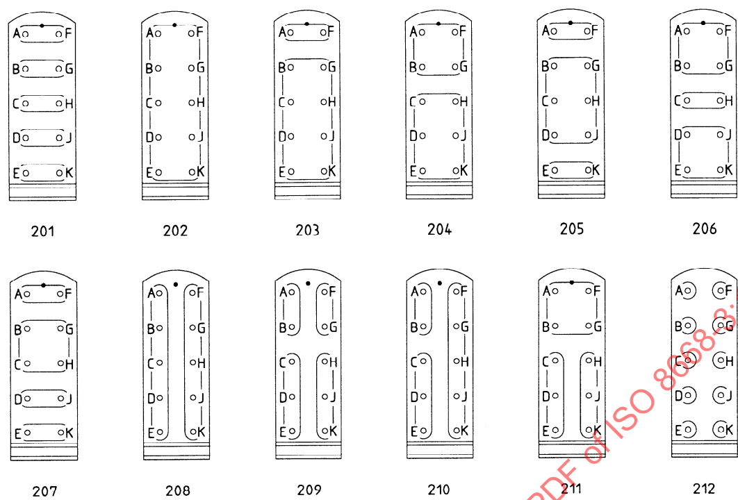
Figure 16 — Size B modules
