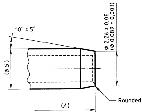
Figure 11 — Detail of the crimping shank of the size 16 contact
