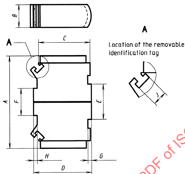
Figure 2 — Feedthrough module
