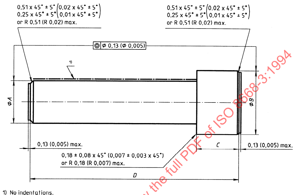
Figure 13 — Sealing plug
