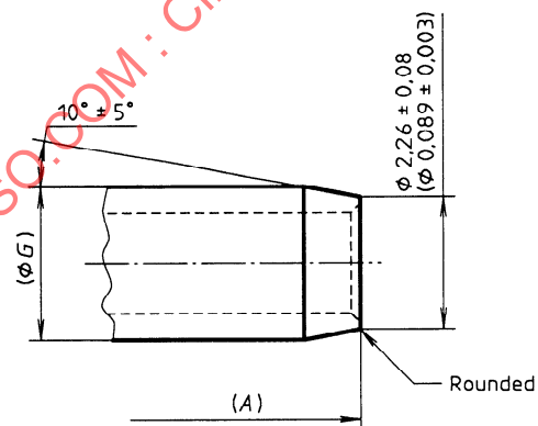
Figure 10 — Detail of the crimping shank of the size 16 contact
