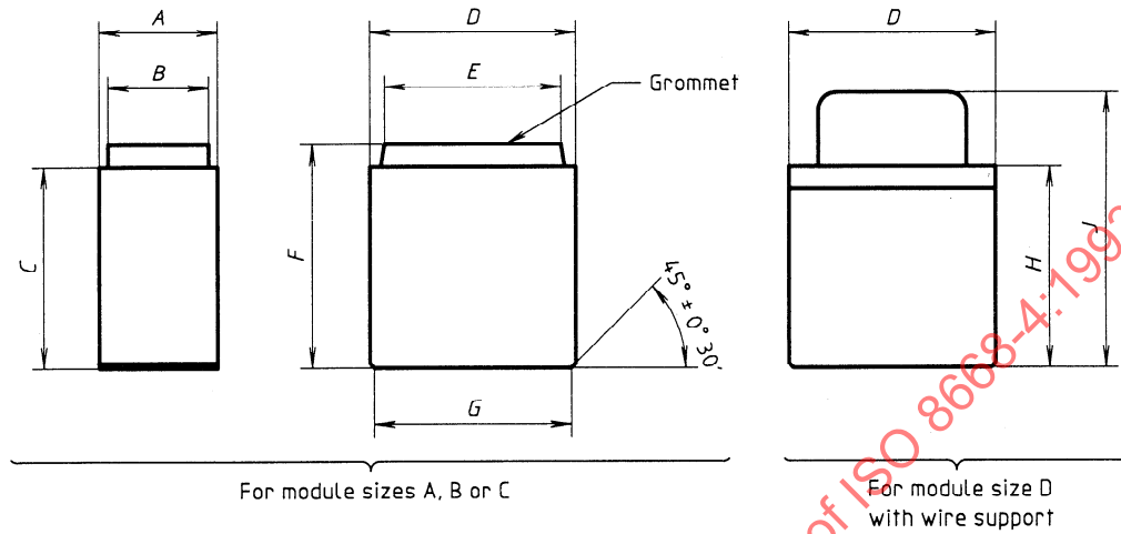
Figure 1 — Feedback modules
