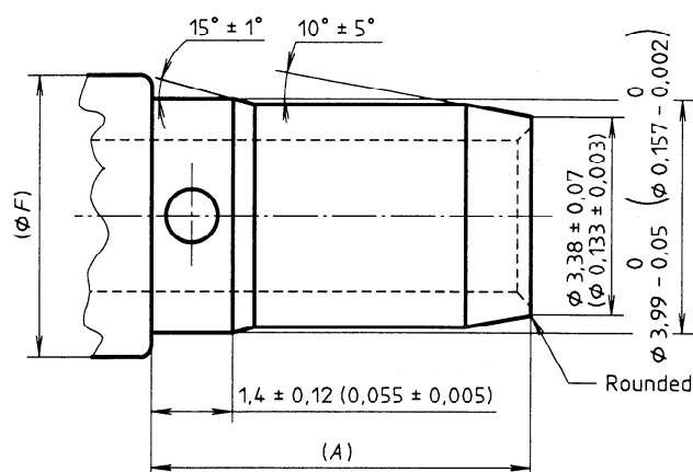
Figure 11 — Detail of the crimping shank of the size 16 contact
