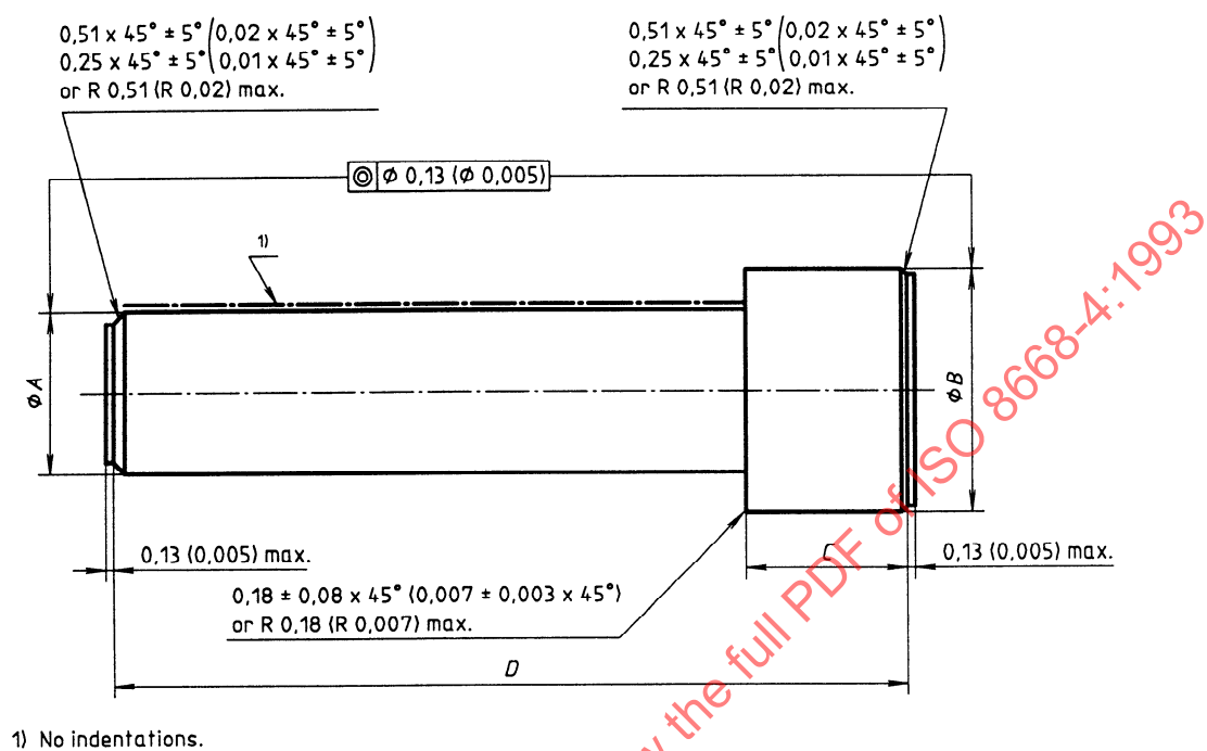
Figure 12 — Sealing plug
