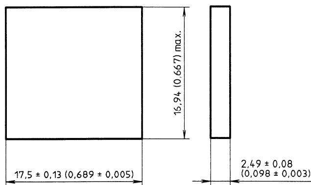
Figure 6 — Spacers (code ER)
