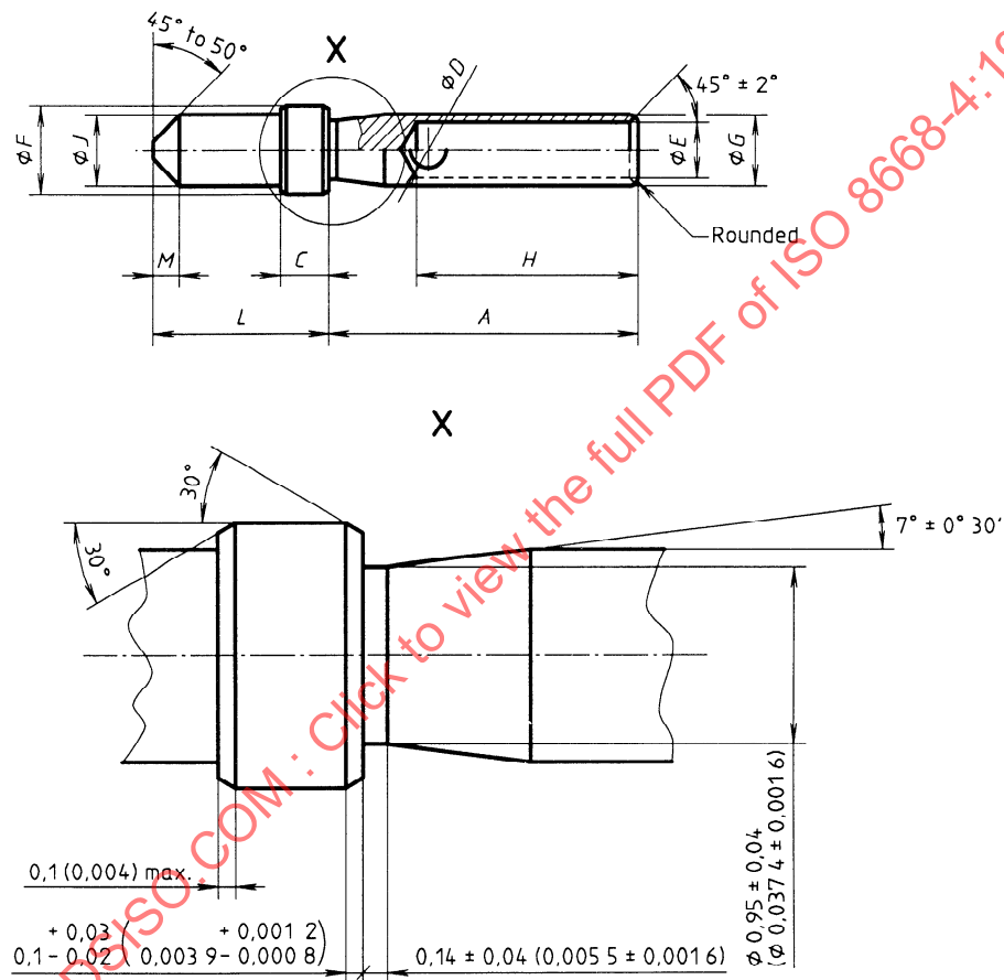
Figure 8 — Contact, size 22
