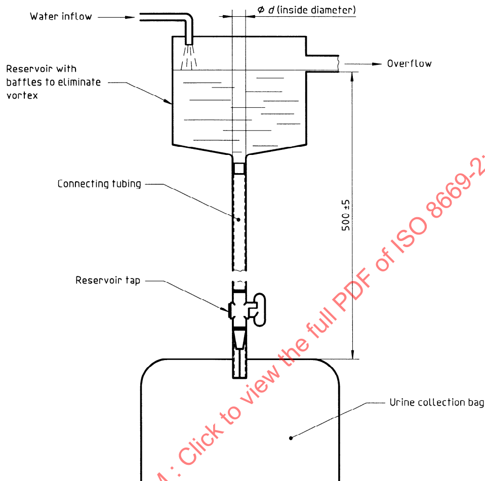
Figure 1 — Filling system for determination of test volume
