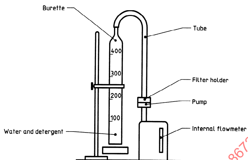
Figure E.1 — Flowrate calibration apparatus
