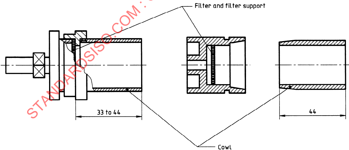
Figure 1 — Filter holders
