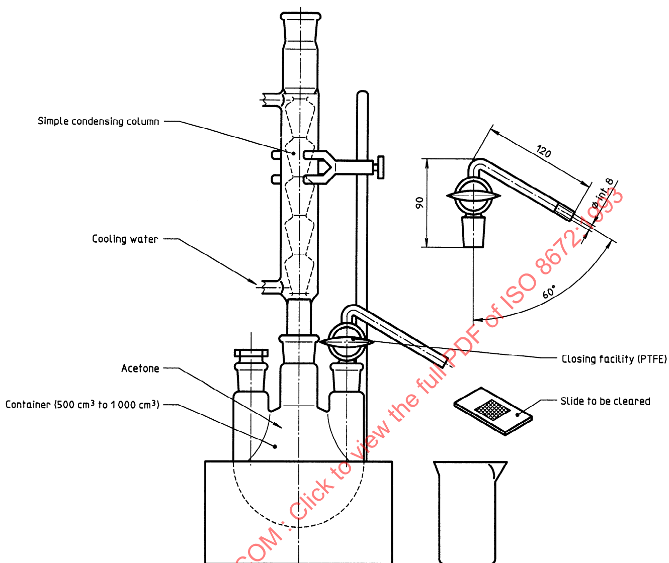
Figure A.1 — Condensing column
