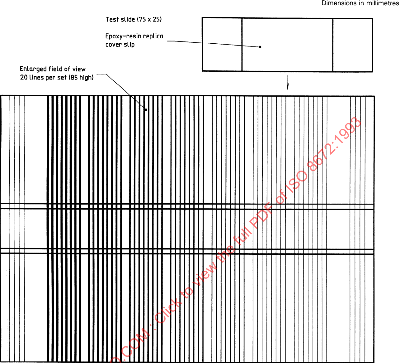
Figure C.1 — HSE/NPL test slide
