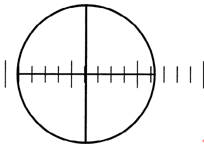
Figure B.1 — Superimposed eyepiece graticule and stage micrometer
