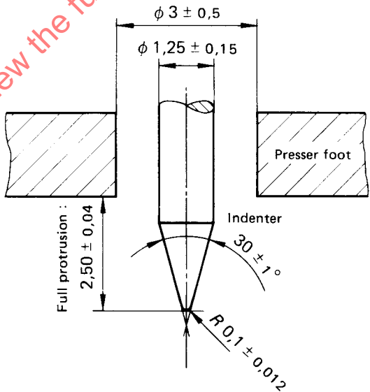
FIGURE 2 — Indenter for type D durometer
