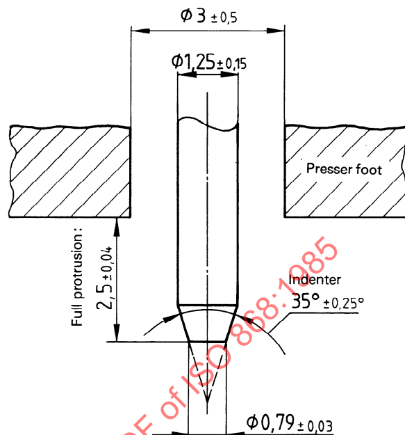
Figure 1 — Indenter for type A durometer
