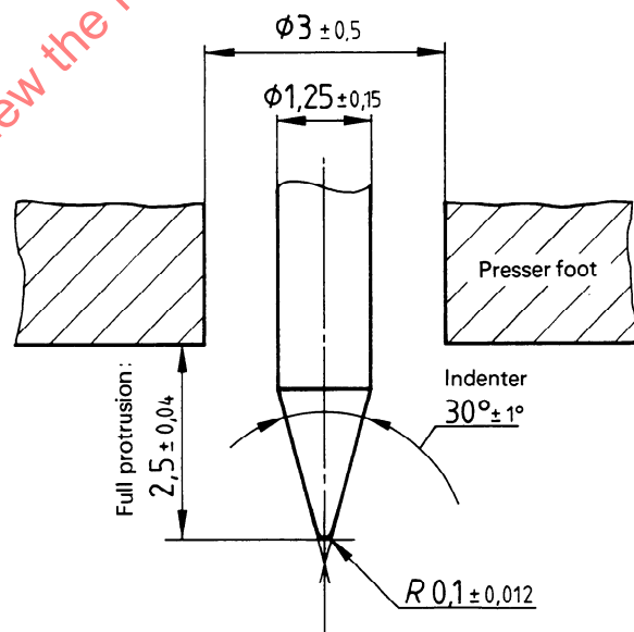
Figure 2 — Indenter for type D durometer
