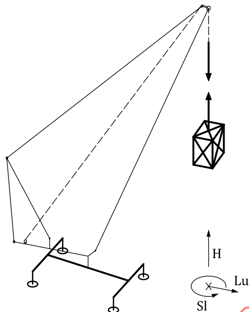
Figure A.3 — Wheeled mobile latticed boom crane (on outriggers)
