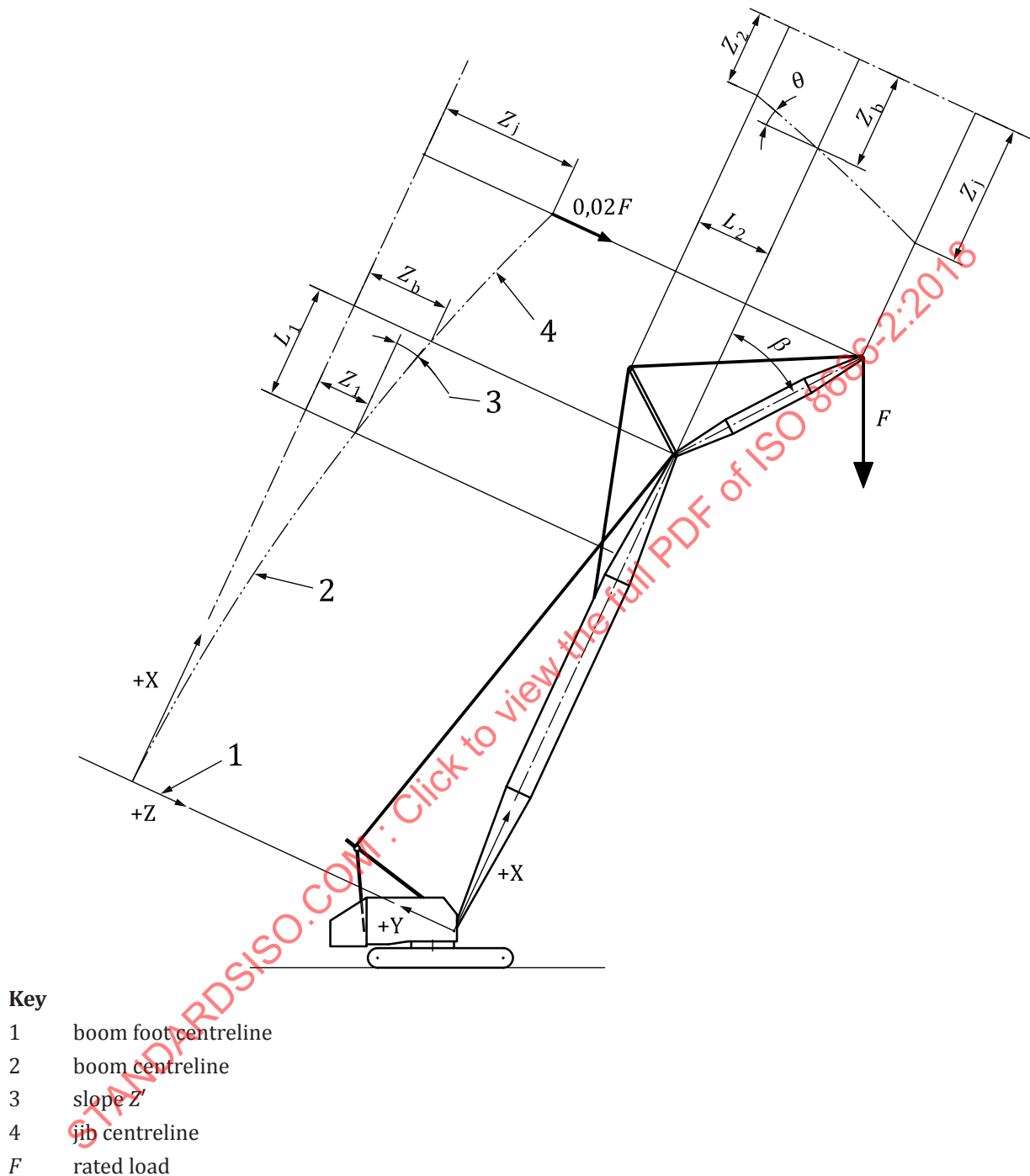
Figure 1 — Terms and symbols related to deflection measurement — Lattice jib with fly jib
