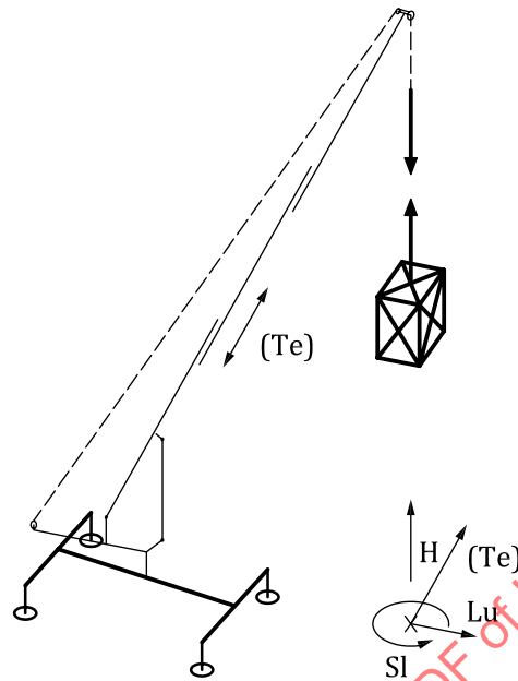
Figure A.4 — Wheeled mobile telescopic boom crane (on outriggers)
