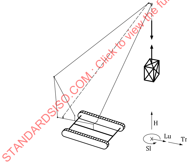
Figure A.1 — Track-mounted (crawler) latticed boom crane
