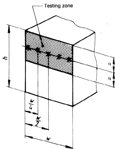
Figure 2 — Hardness testing
