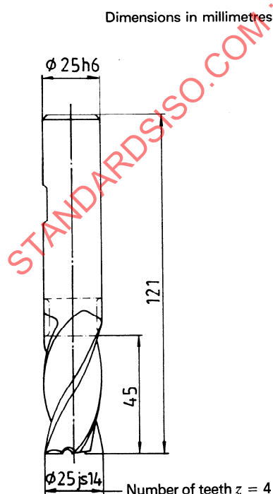
Figure 5 — End mill (see ISO 1641-1)
