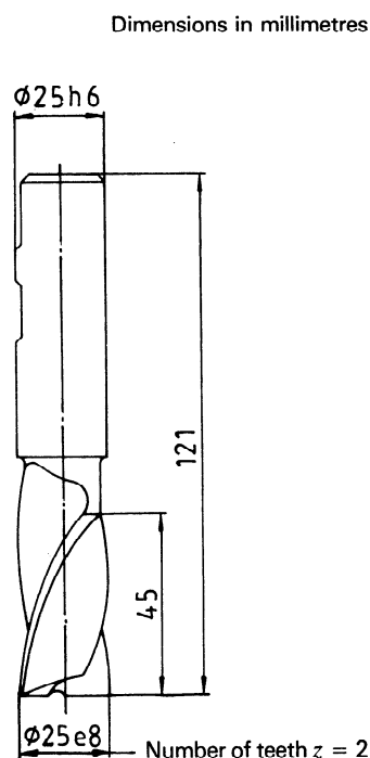
Figure 6 — Slot drill (see ISO 1641-1)
