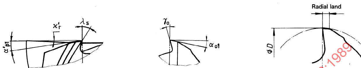
Figure 7 — Tool geometry
