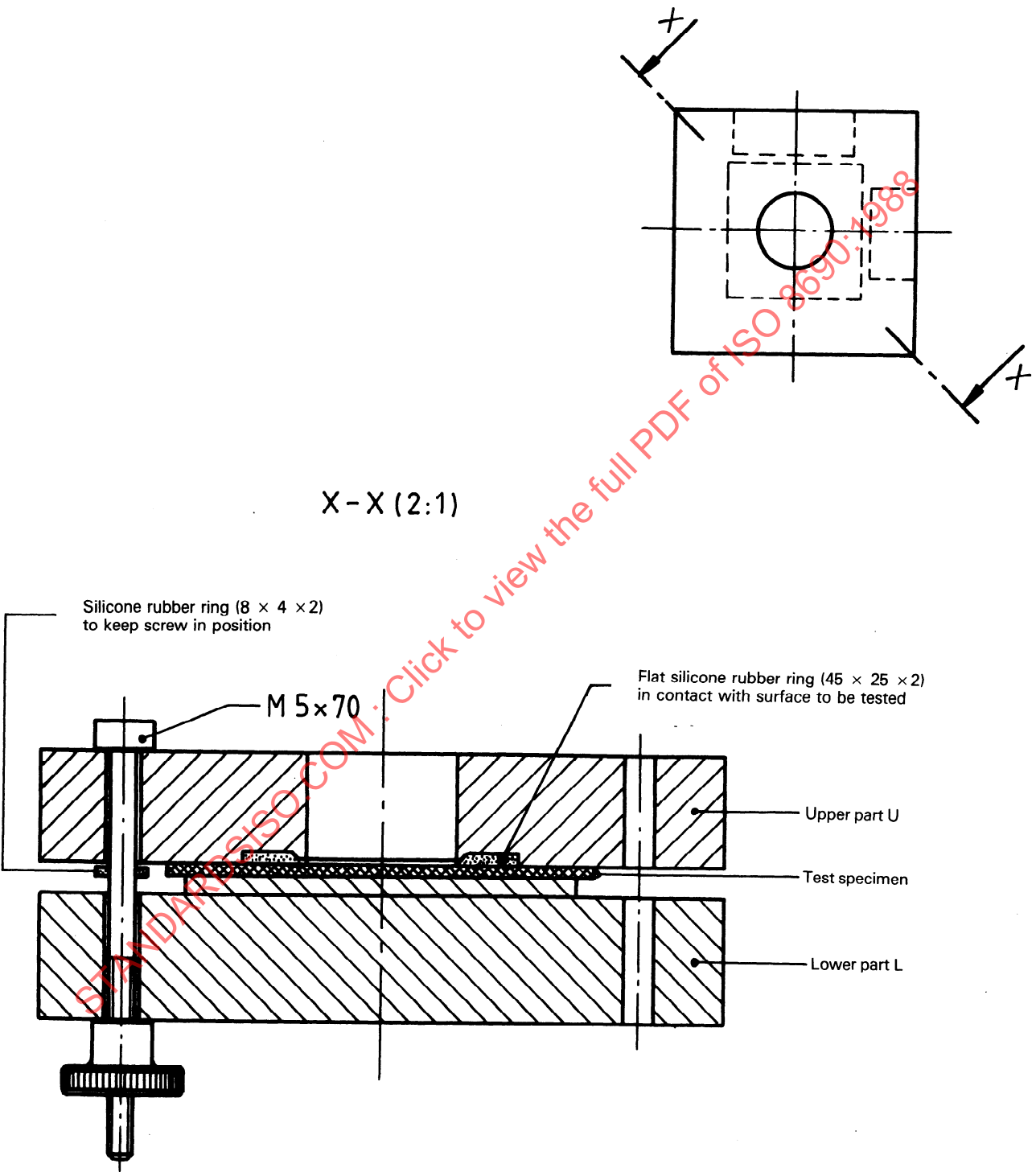
Figure 2 — Holder for contamination of test specimen (see also figures 5 and 6)
