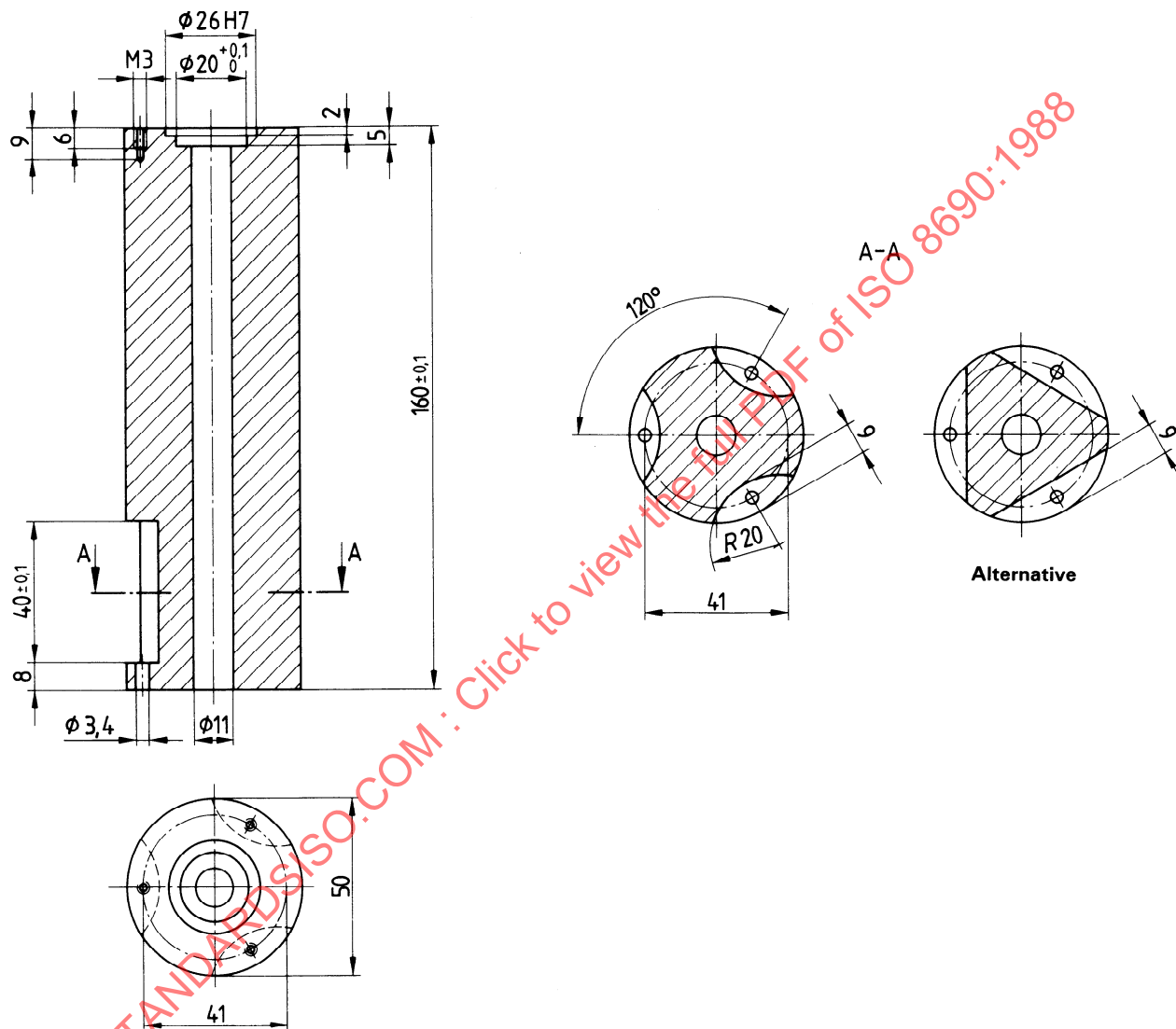
Figure 8 — Stirrer support column
