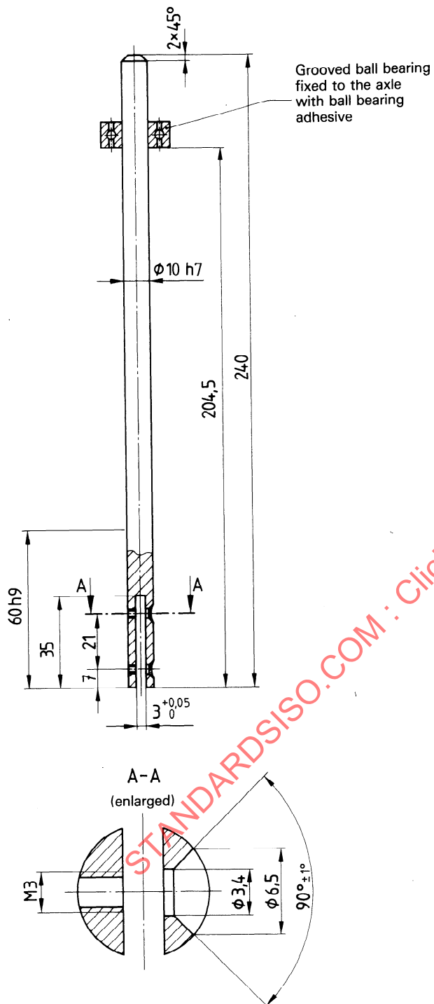
Figure 9 – Stirrer axle
