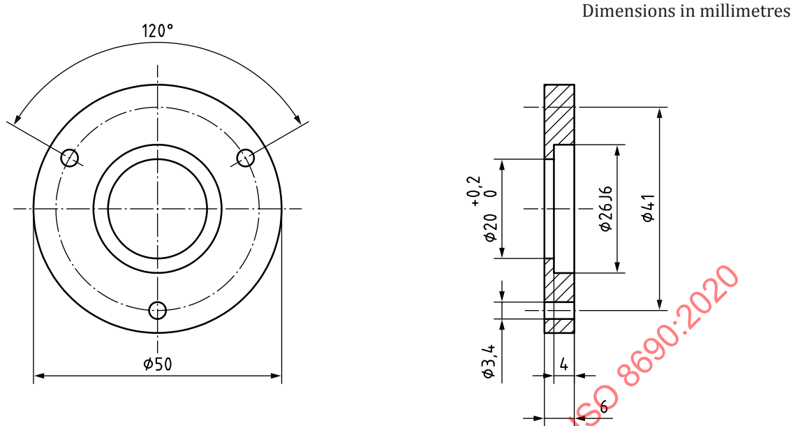
Figure B.4 — Mounting support for ball bearing
