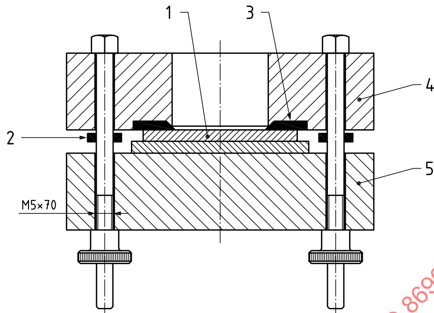
b) Holder for contamination of test specimen; drawn in profile (insertion of test specimen, see also Figures A.1 and A.2 )
