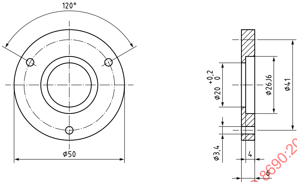
Figure B.4 — Mounting support for ball bearing
