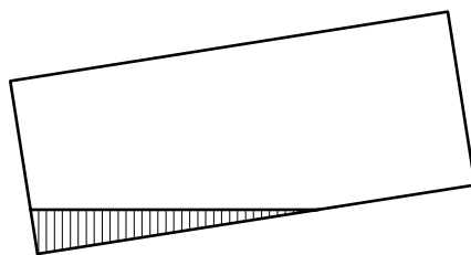
Figure A.3 — Example of a single liquid in contact with only three bulkheads
