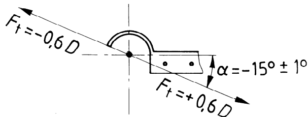
Figure 1 — Dynamic test
