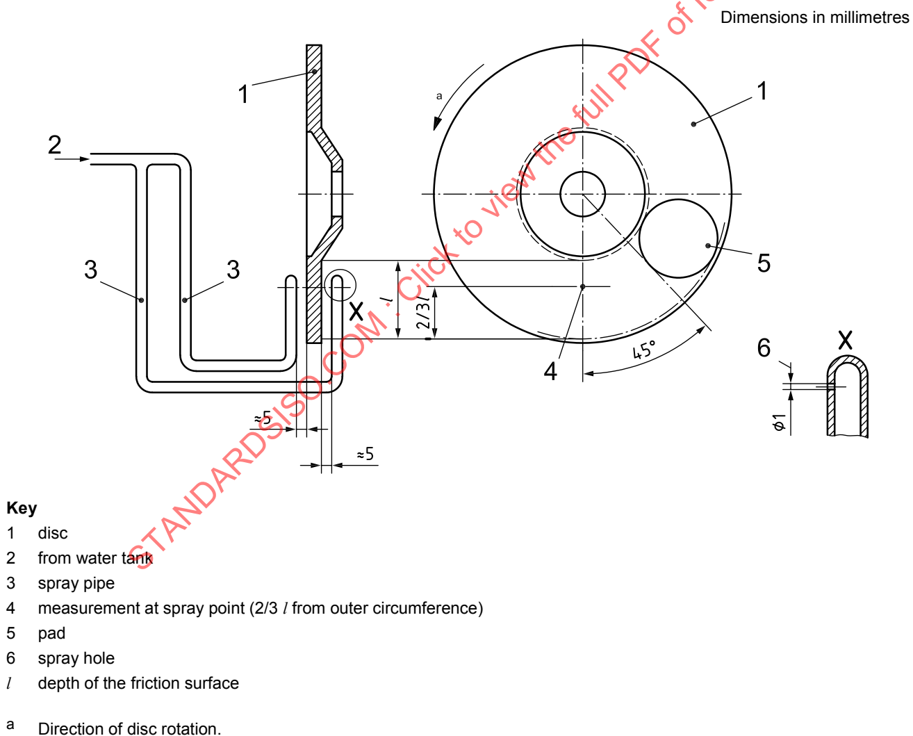
Figure 2 — Water spray equipment for disc brakes
