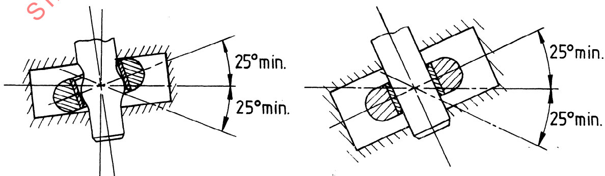
Figure 5 — Rotation angle
