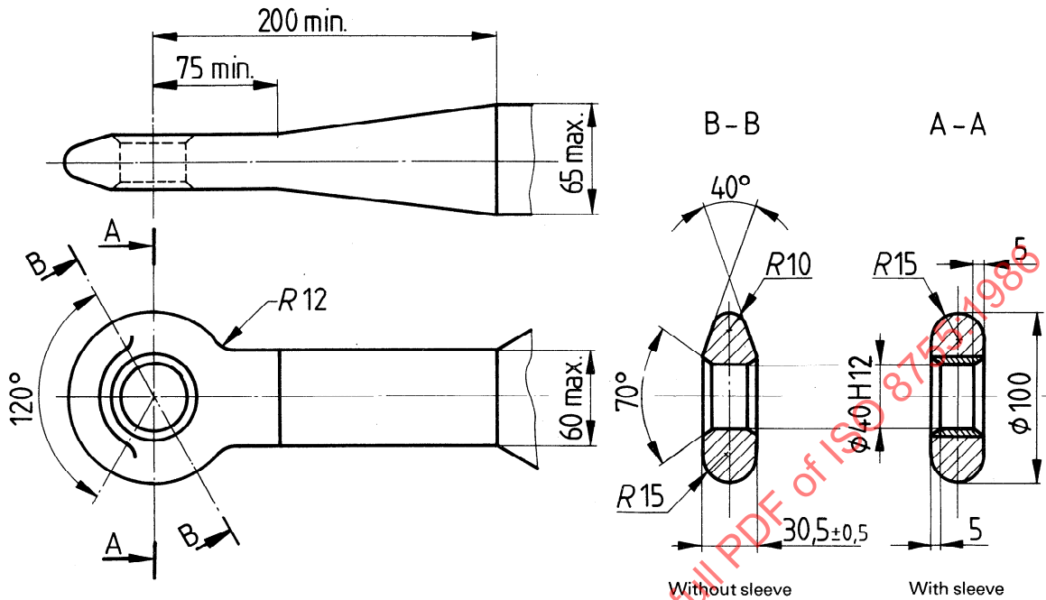
Figure 1 — 40 mm drawbar eye
