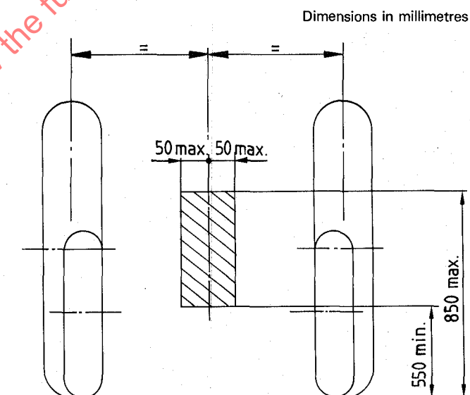
Figure — Location of power take-off
