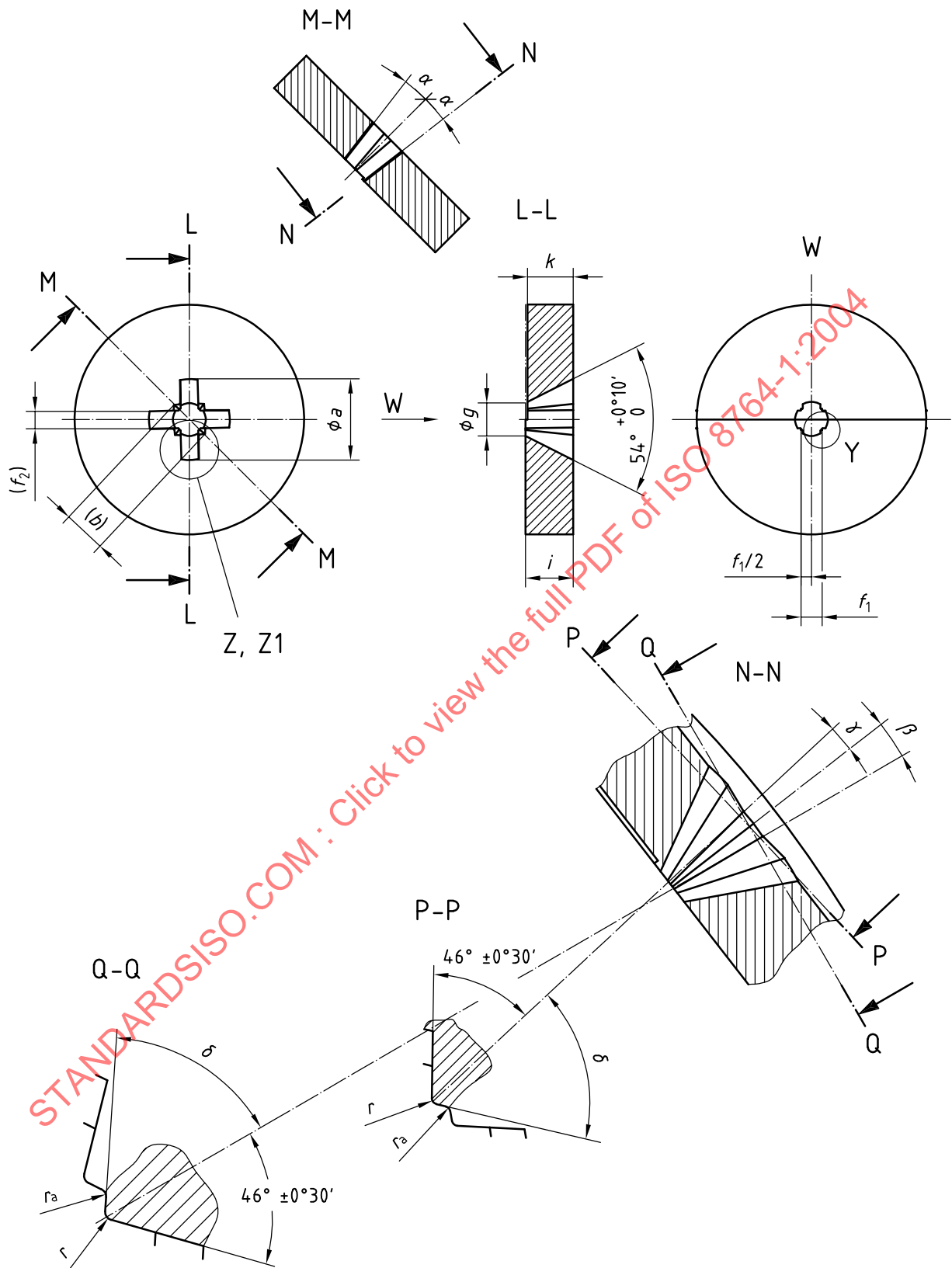
Figure B.2 — Inspection gauge for form PZ tips
