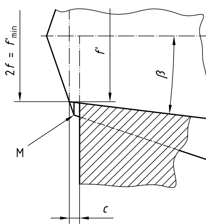
Figure A.2 — Detail of section H-H of Figure 3 (with tip mounted)
