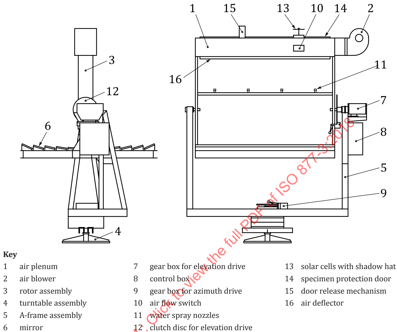
Figure 2 — Schematic diagram of test apparatus with dual-axis tracking
