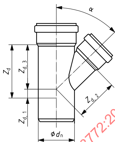
Figure 19 — Reducing branch
