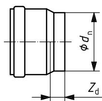
Figure 22 — Push-fit socket for butt-fusion to pipe end
