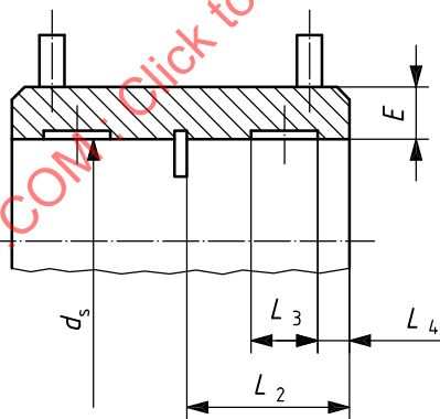
Figure 7 — Electrofusion socket
