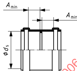
Figure 13 — Coupler
