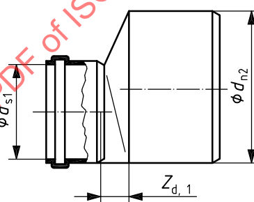
Figure 15 — Reducer
