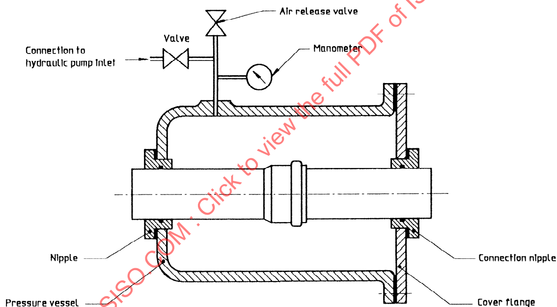
Figure C.1 — Test equipment for external hydrostatic pressure test
