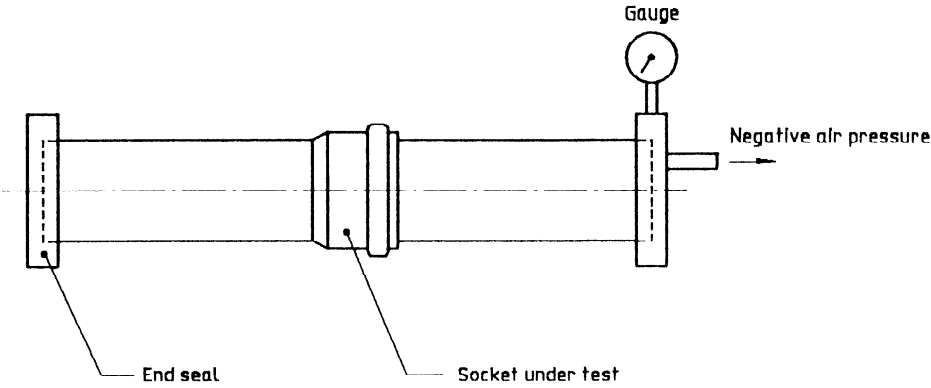
Figure C.2 — Apparatus for the internal negative air pressure test
