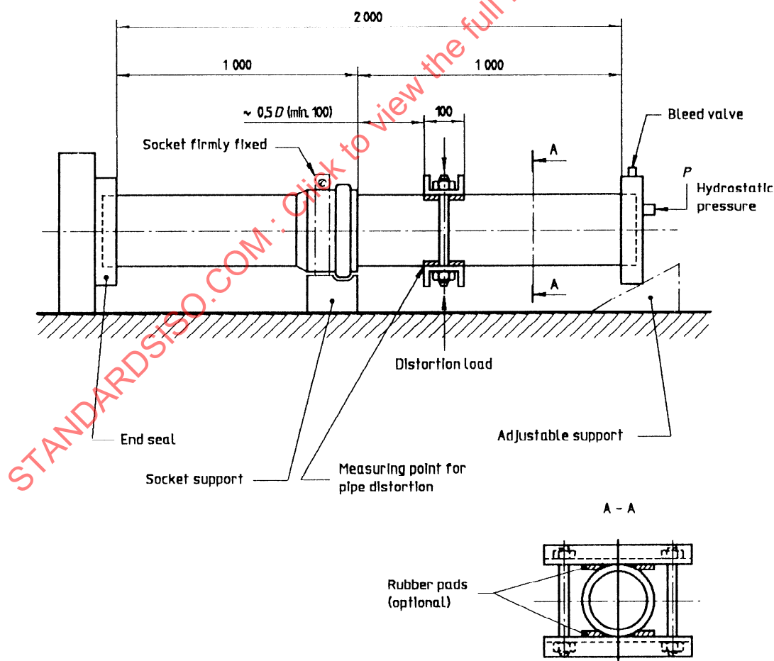
Figure D.1 — Diameter distortion test equipment
