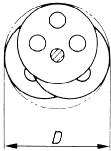
Figure 2 — Effective diameter of discs
