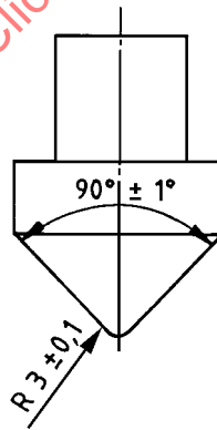
Figure 16 — Impact striker
