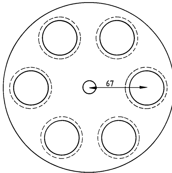
Figure 27 — Holder for jars used in the water vapour permeability test
