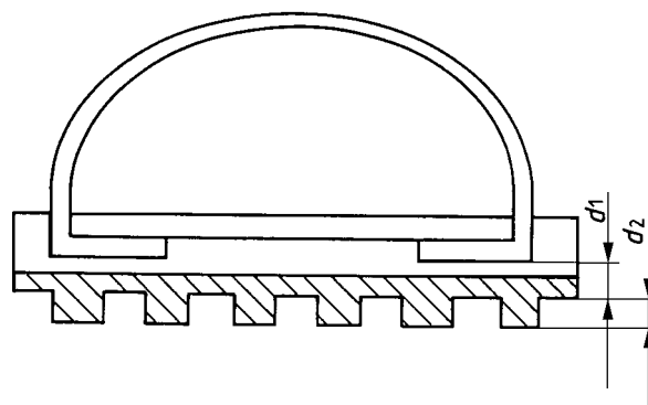
Figure 7 — Multilayered outsoles
