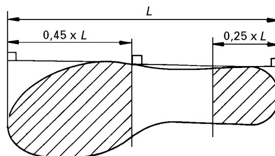
Figure 5 — Cleated area
