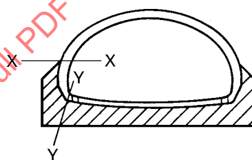
d) Type d: Strobel-stitched with cemented-dished, direct-injected or vulcanized outsole
