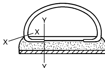
g) Type g: multilayered sole with moulded-on sole, moulded unit or built unit
