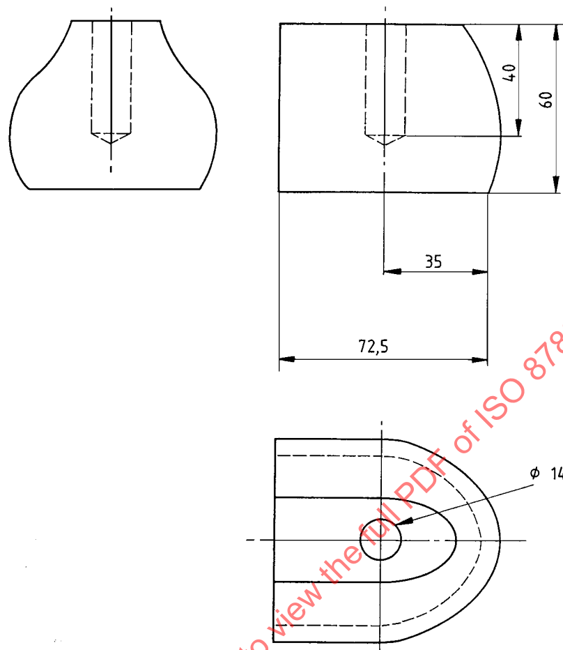
Figure 25 — Test punch for energy absorption test
