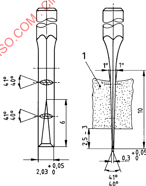
Figure 31 — Cutting tool
