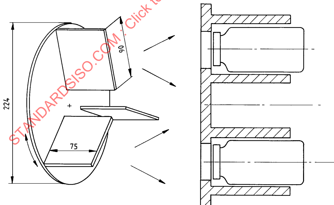
Figure 28 — Schematic diagram of apparatus to be used in the water vapour permeability test
