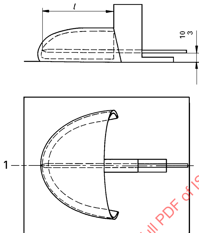
Figure 15 — Measurement of internal toecap length
