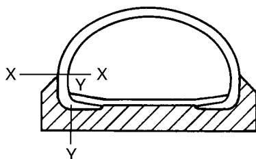
c) Type c: conventional lasting with direct-injected or vulcanized outsole or cemented-dished outsole
