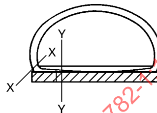
b) Type b: conventional lasting with close-trimmed outsole
