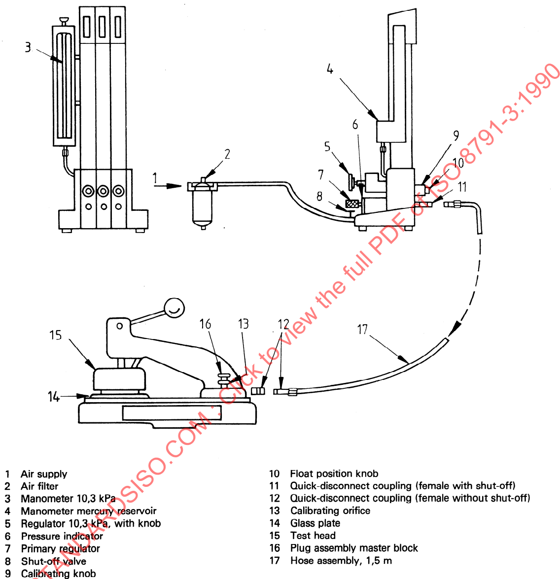
Figure 1 — Sheffield roughness tester
