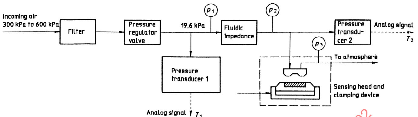
Figure E.1 — Flow diagram of an impedance instrument showing additional transducer
