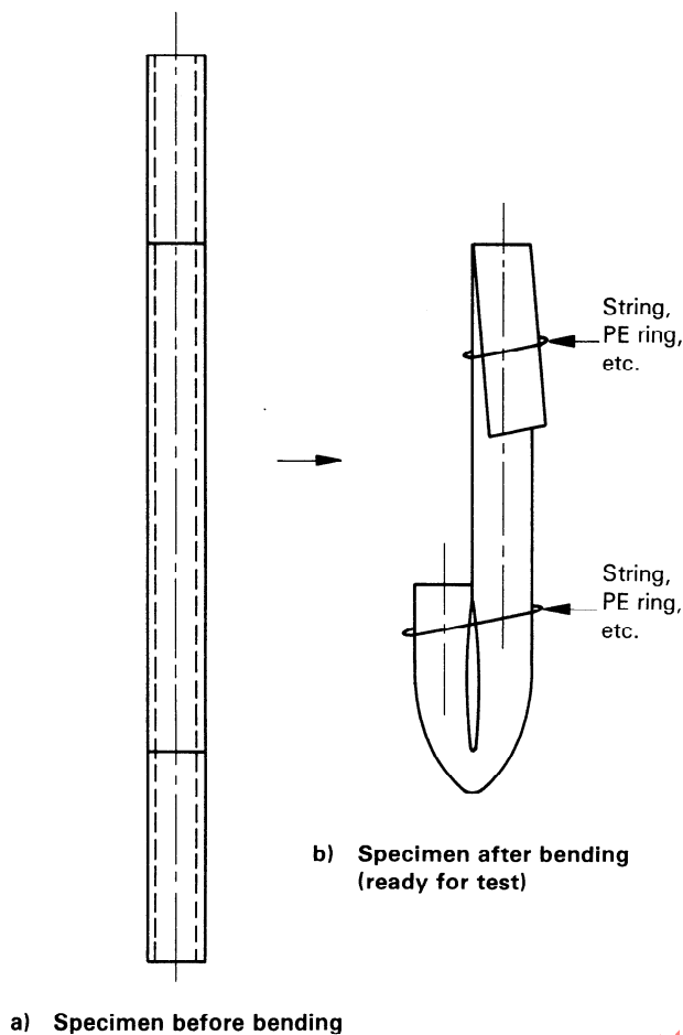
Figure 2 — Preparing the U-bends
