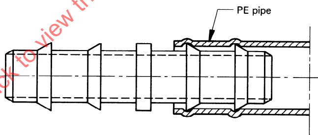
Figure 1 — In-line connector
