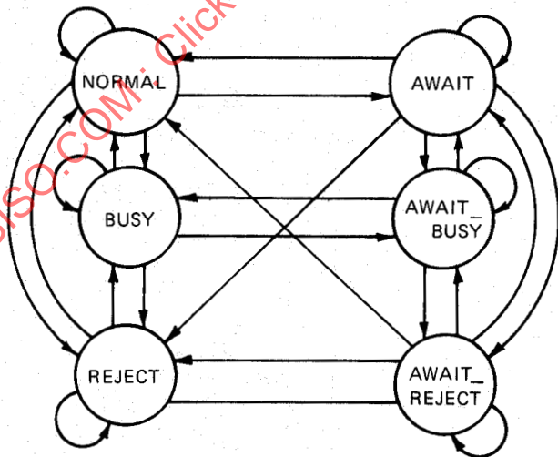
(b) Information Transfer (Connected) States
