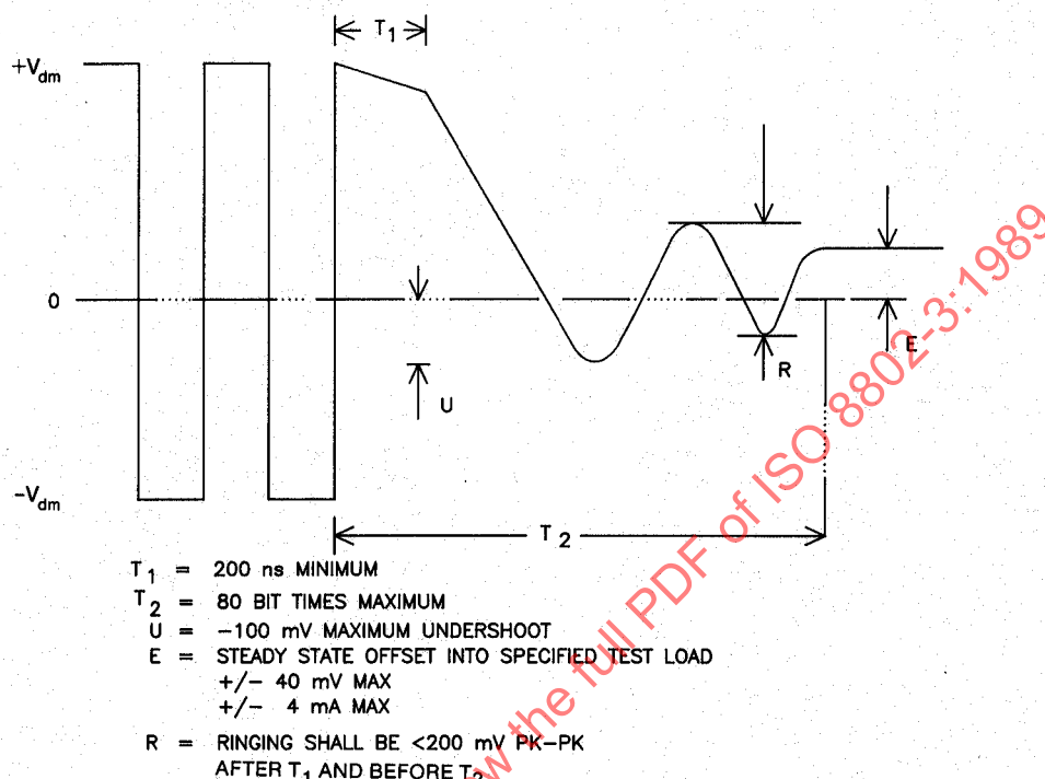
Fig 7-12 Generalized Driver Waveforms
