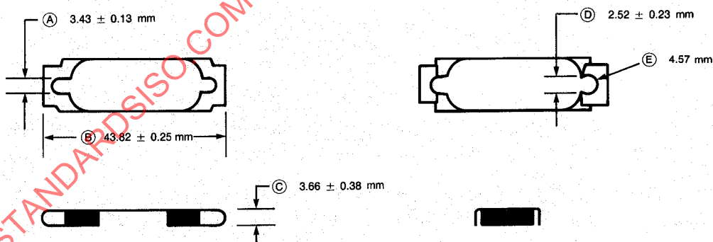
Fig 7-19 Connector Slide Latch
