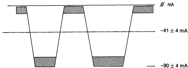
Fig 8-5 Recommended Driver Current Levels
