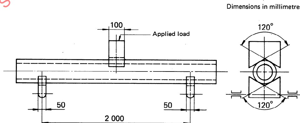
Figure 3 — Loading in longitudinal bending test
