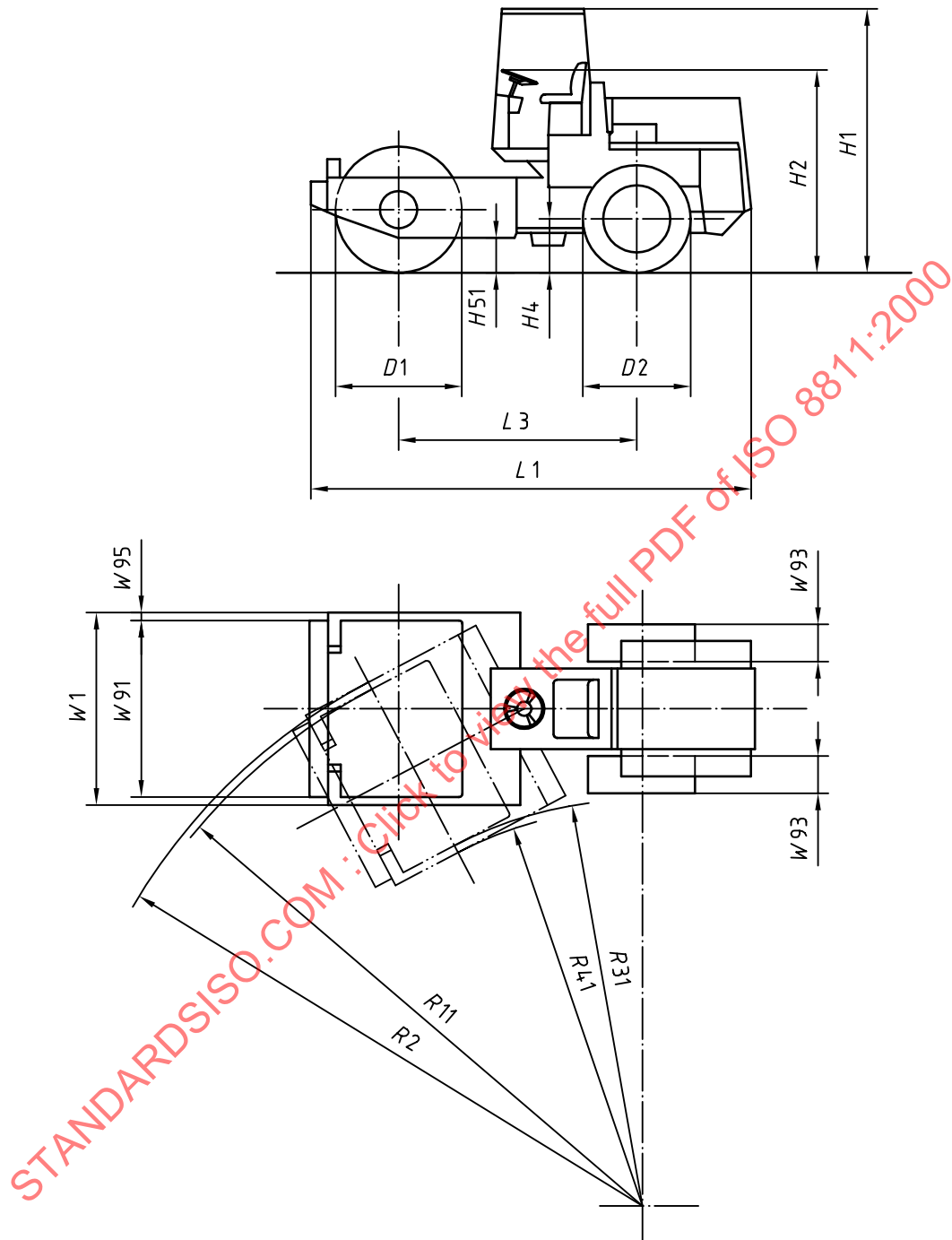
Figure 16 — Dynamic single-drum, dual-wheel roller with pivot-articulated steering
