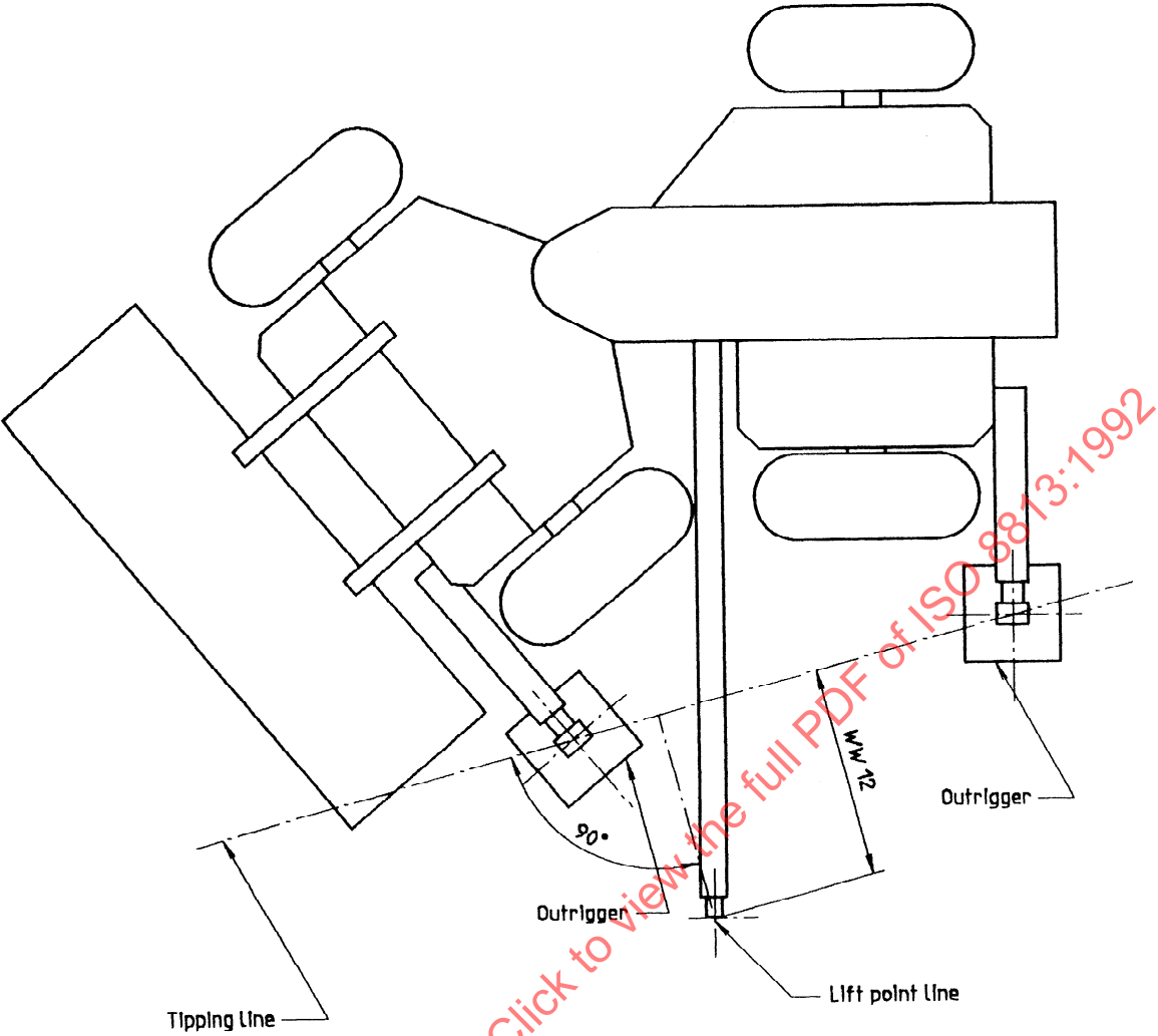
Figure 7 — Articulated machine using outriggers; steered left
