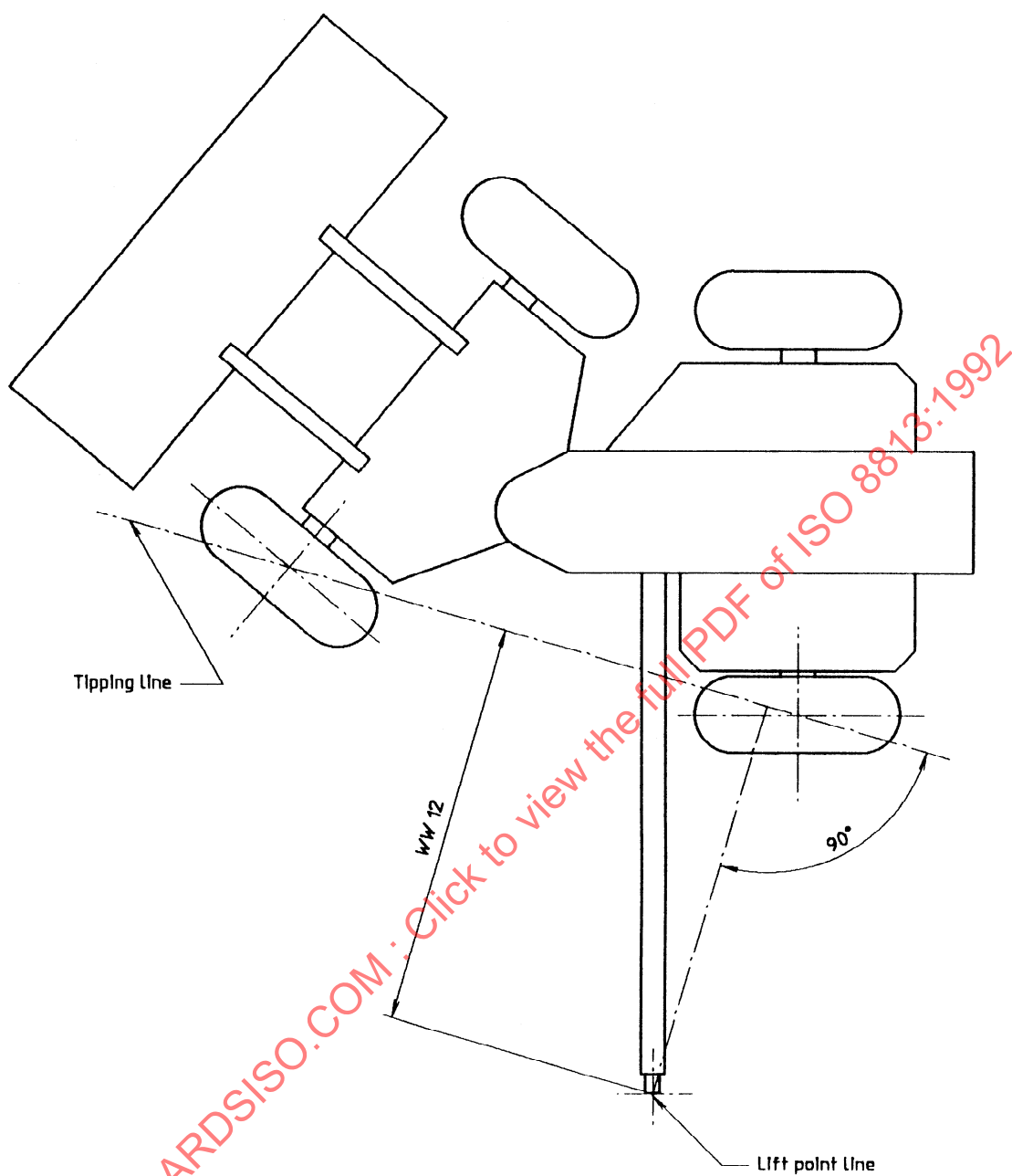
Figure 5 — Articulated wheeled machine steered right; non-oscillating axle
