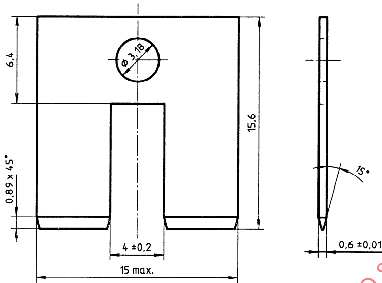
Figure 2 — Test slug
