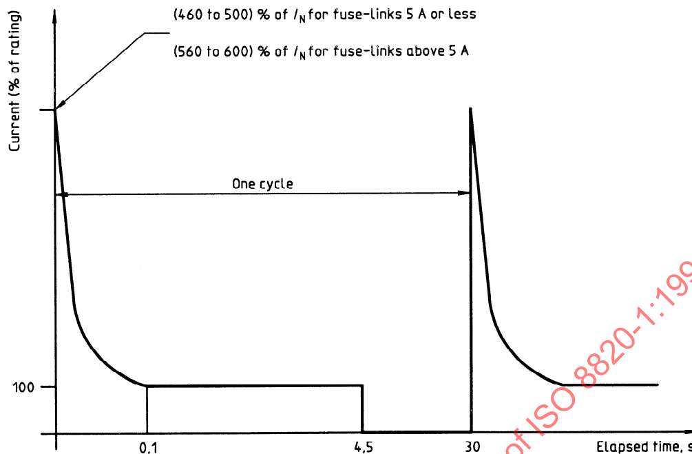
Figure 4 — Transient current cycling
