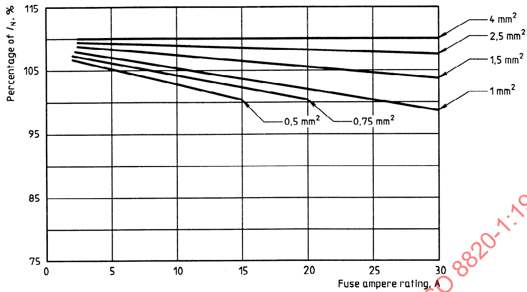
Figure A.2 — Change in fuse-link current-carrying capacity for various sizes at 24 °C
