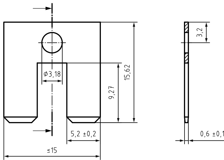
Figure 3 — Test dummy for Type C fuse-links
