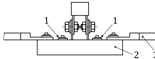
a) Test fixture for types A1, A1S, A2, A3 and A4
