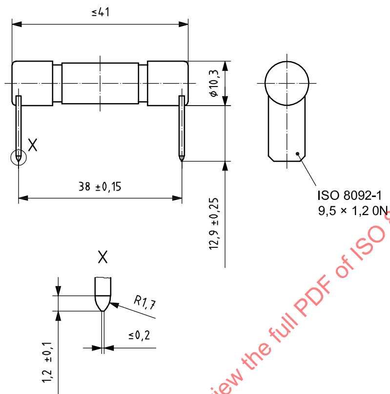
Figure 3 — Fuse-links with I_R < 35 A
