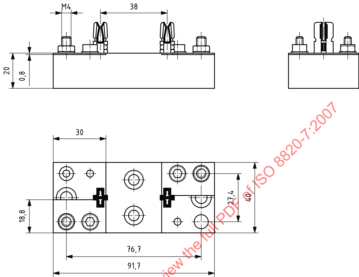
Figure 6 — Test fixture for fuse-links with I_R < 35 A
