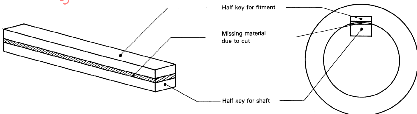
Figure C.1 — Half-height key set
