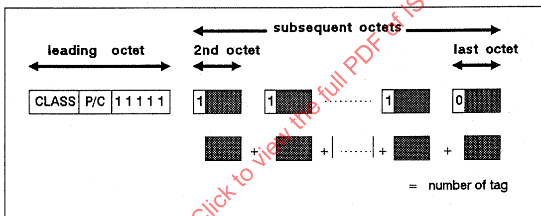
Figure 4 — Identifier octets (high tag number)
