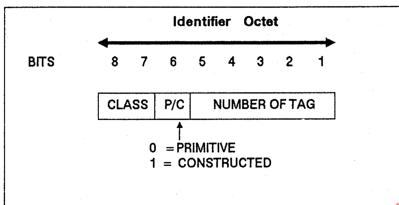
Figure 3 — Identifier octet (low tag number)
