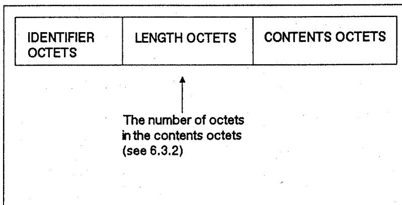
Figure 1 — Structure of an encoding
