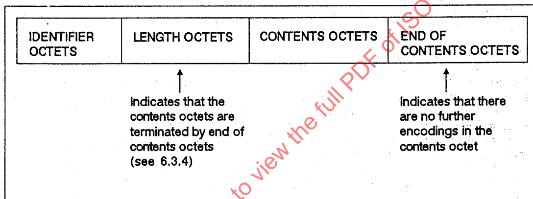
Figure 2 — An alternative constructed encoding
