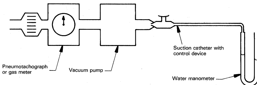
Figure 3 — Apparatus for residual vacuum test
