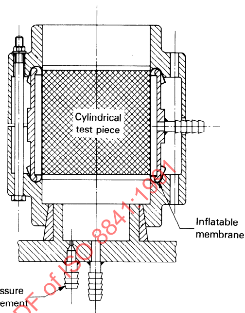
Figure 3 — Test piece holder
