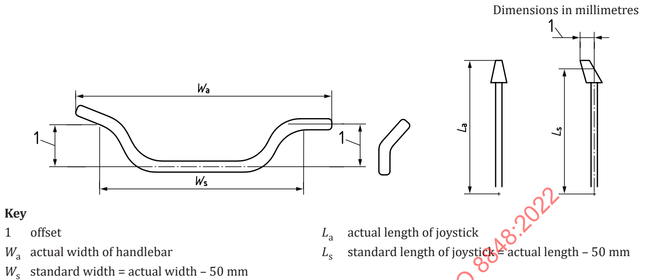
Figure 7 — Control elements
