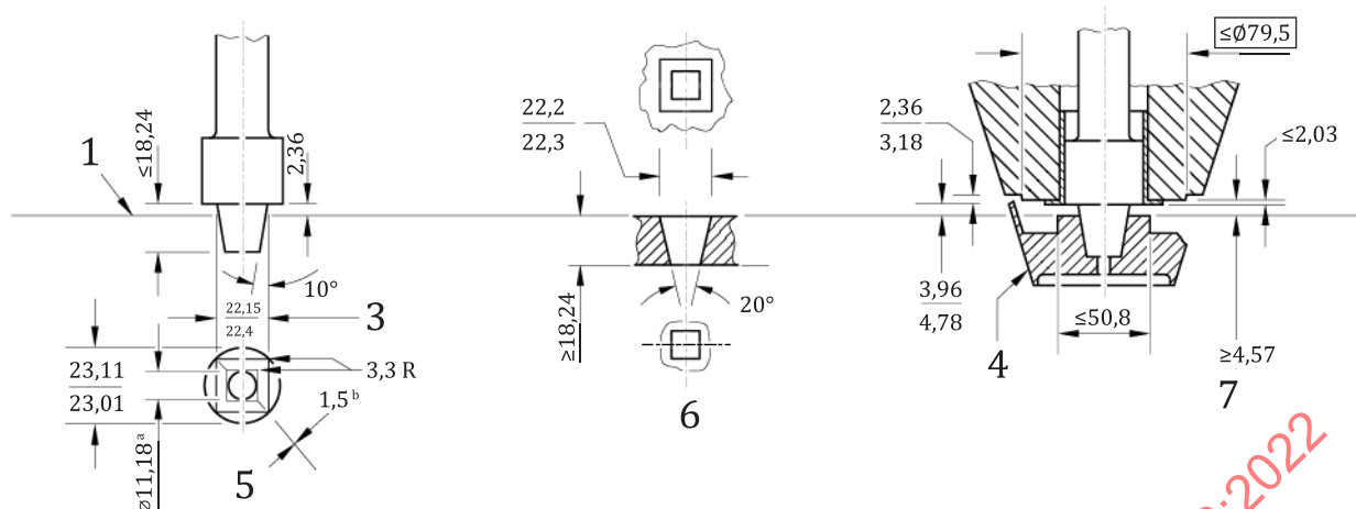
c) Tapered square shaft and steering wheel hub
